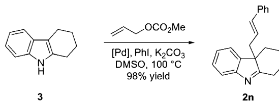
Scheme 4. Three-Component Cinnamylation Reaction
