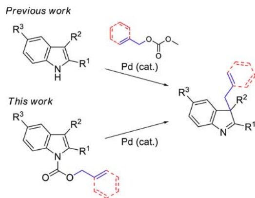
Scheme 1. Decarboxylative Allylation of Indole
