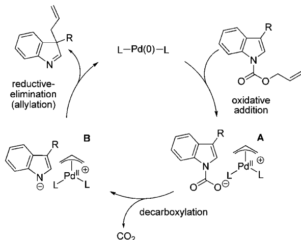
Scheme 2. Catalytic Cycle for Decarboxylative Allylation
