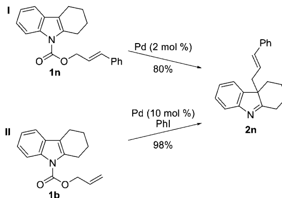
Scheme 3. Formation of Cinnamyl Product a
