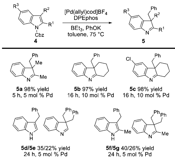
Scheme 5. Substrate Scope of Benzylation Reaction a
